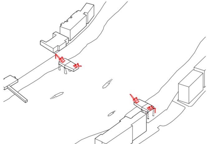
BALANCE CANTILEVER SEGMENTAL CONSTRUCTION
