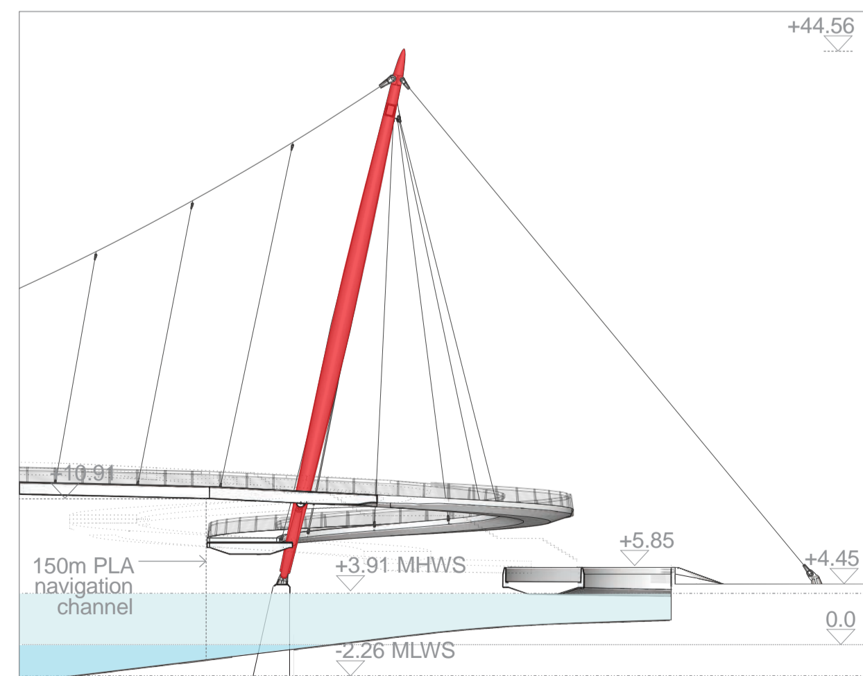
Long section at landing
