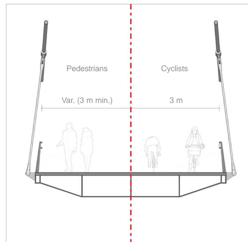
Cross section through deck
