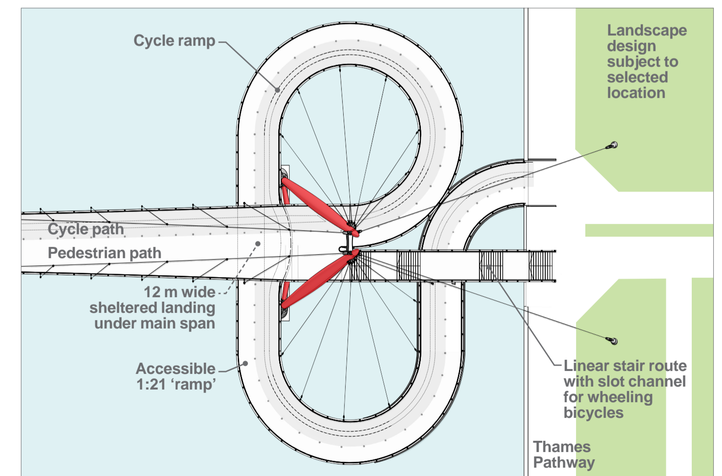
Plan at landing
